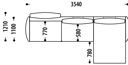
2MrL-OTPL L+150mm
